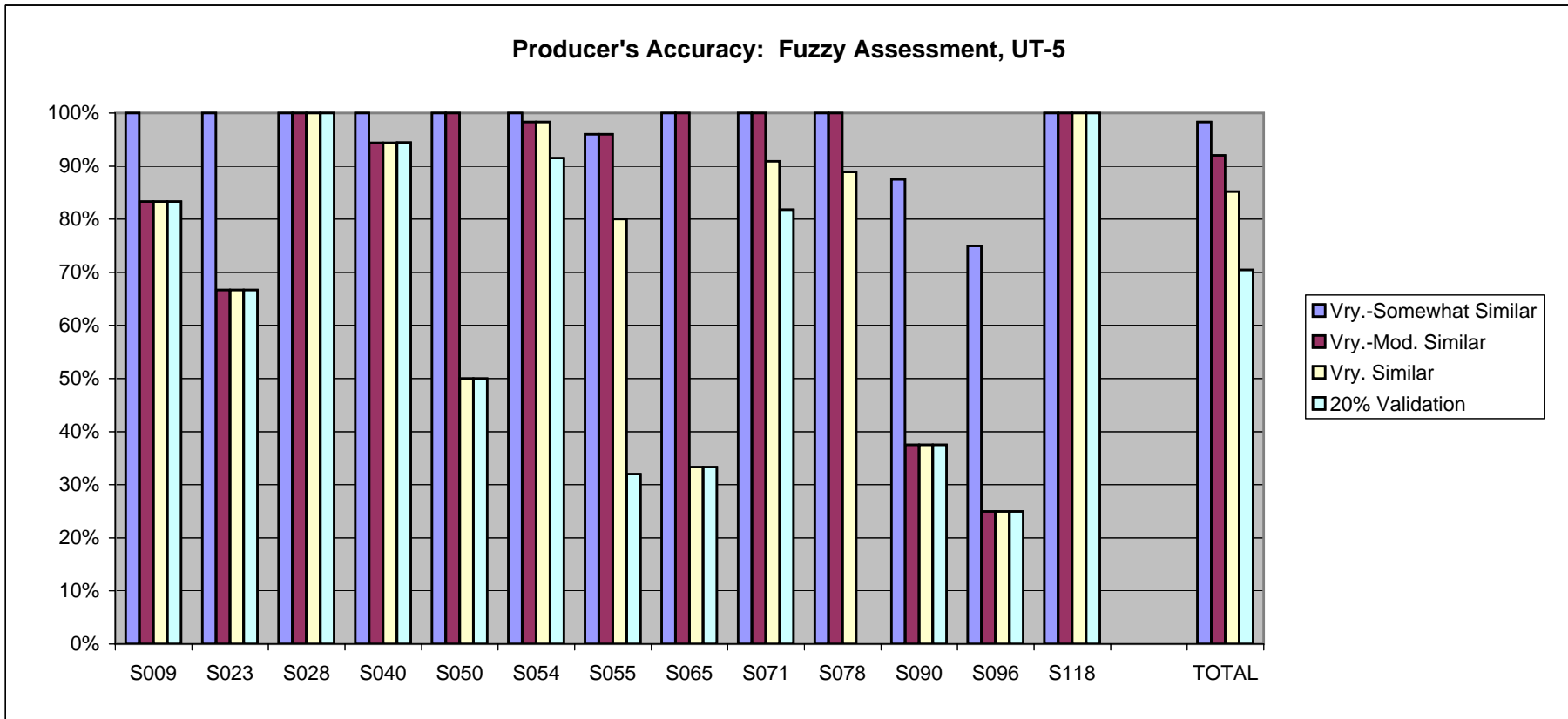
Graph 2. Producer's Accuracies Relative to Adjusted Fuzzy Set Assessment
